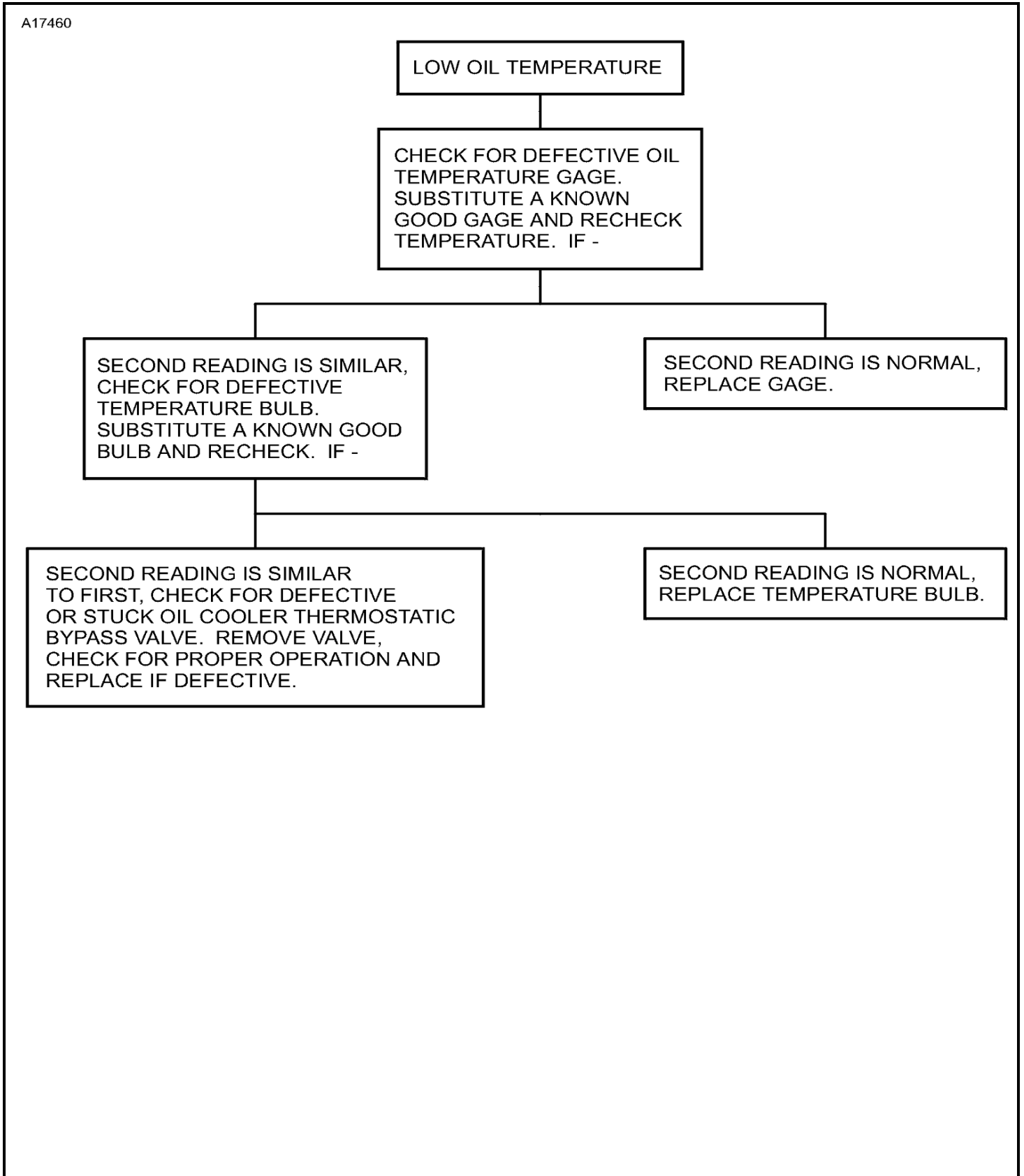
Figure 101 : Sheet 3 : Oil Indicating System Troubleshooting Chart
